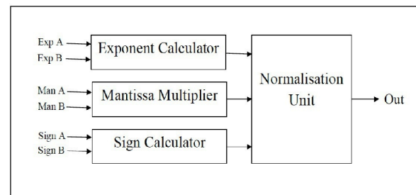
Fig.3. Normalization of sign, exponent and mantissa
