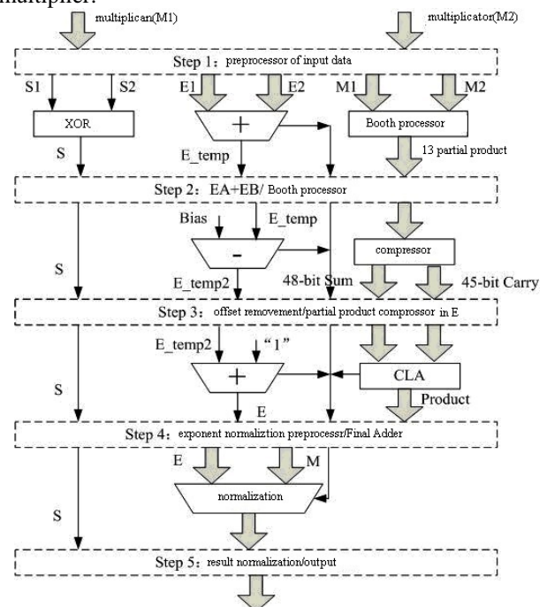
Fig.4. Algorithm for floating point multiplication
