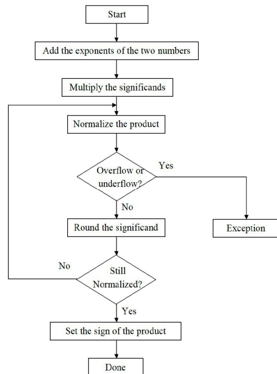
Fig.5. Floating point multiplier flow graph
