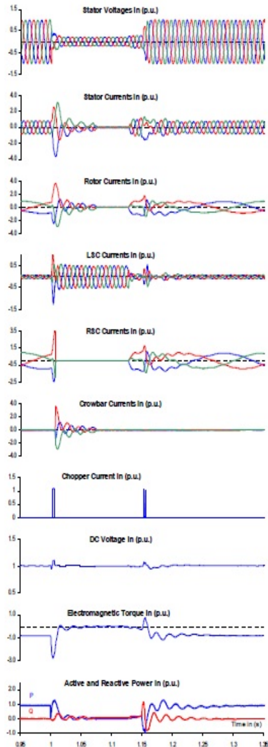
Fig.7. FRT example with only one crowbar period by using both crowbar and DC-link chopper as well
