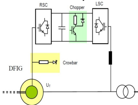
Fig.5. DFIG base system extended by FRT protection devices
