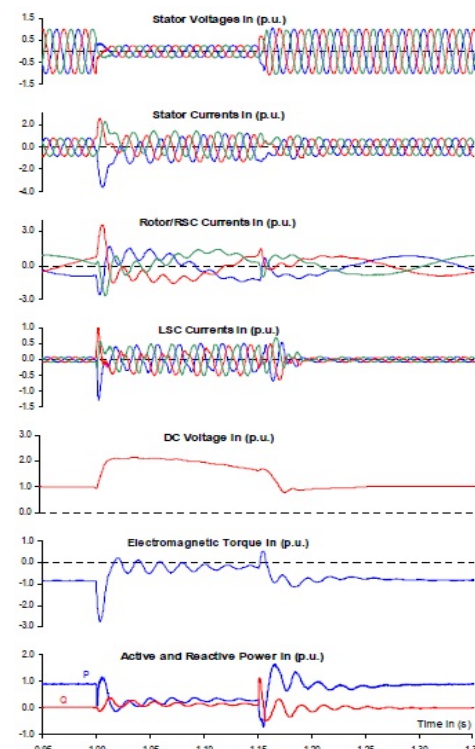
Fig.4. Behavior of DFIG wind turbine during a three phase grid short circuit without FRT measures (theoretical case)
