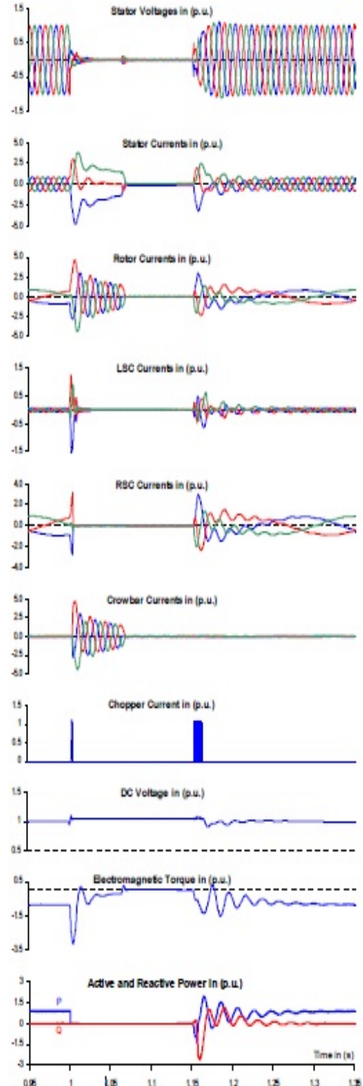
Fig.9. Zero voltage ride through by using both crowbar and DC-link chopper as well
