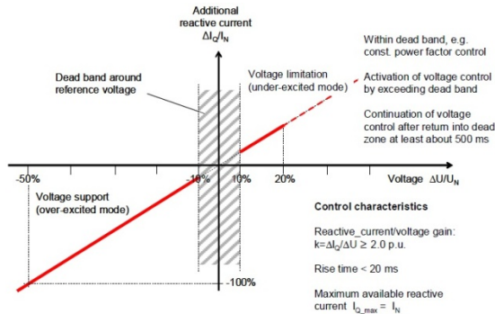
Fig. 2. Characteristic of wind turbine voltage control
