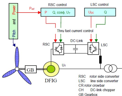
Fig.3. Structure of the DFIG based wind turbine
