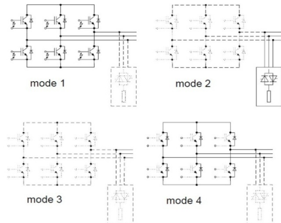
Fig.6. Operating modes of the DFIG rotor side converter
