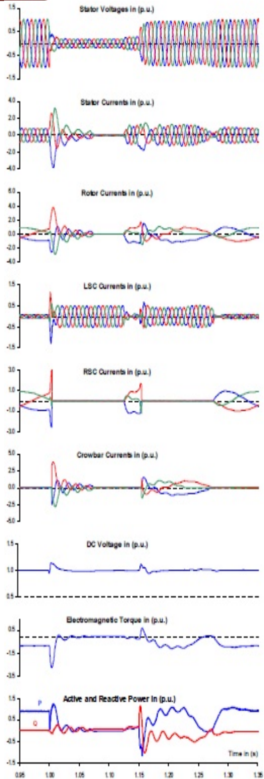
Fig.8. FRT example with a second crowbar period after voltage recovery (no chopper is implemented)
