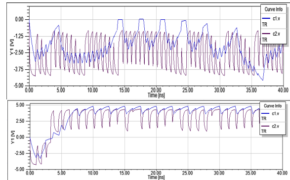
Fig.13. output of the loop filter for standard (in Blue) and proposed (in Red).
