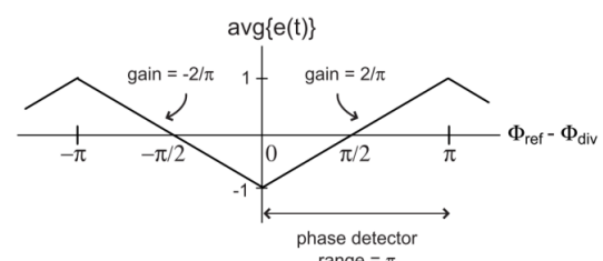
Fig.3. Output Average Value with Phase Error for XOR Phase Detector.
