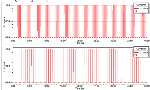
Fig.10. The clock input for tracking 1.2 GHz (above) 0.8 GHz (below).
