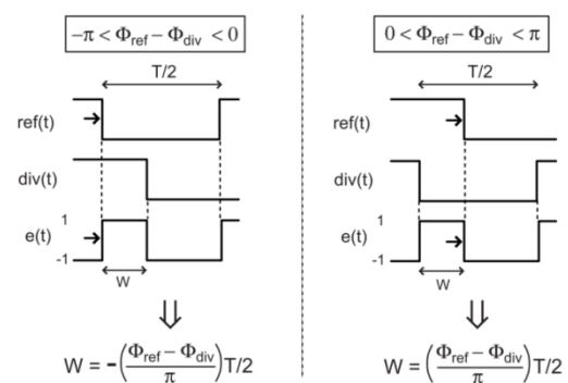
Fig.2. XOR Phase Detector Calculation
