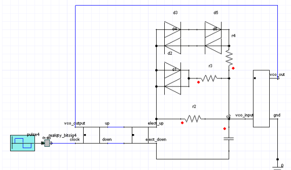
Fig.9. the simulated model of proposed digital PLL.
