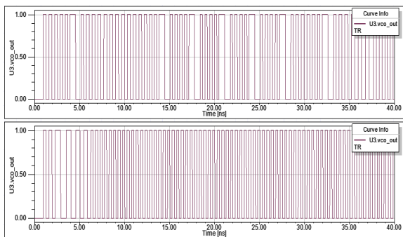
Fig.11. The clock input tracked by standard digital PLL shows a lot of variations and larger time to get locked.
