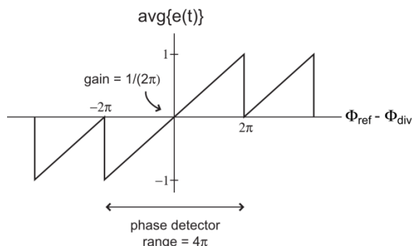
Fig.5. Average Value calculation for PFD.
