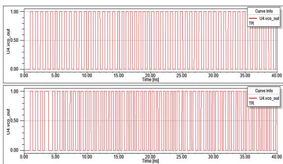
Fig.12. The clock input tracked by proposed digital PLL shows smooth tracking and quick locking.
