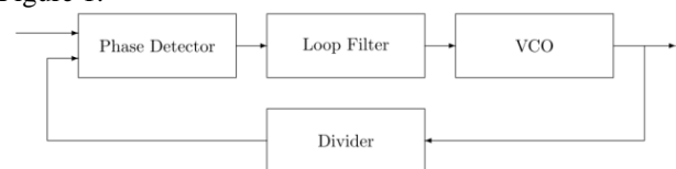
Fig.1. Block Diagram of Basic Digital PLL.
