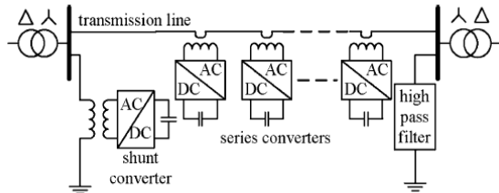
Fig. 3. DPFC configuration.
