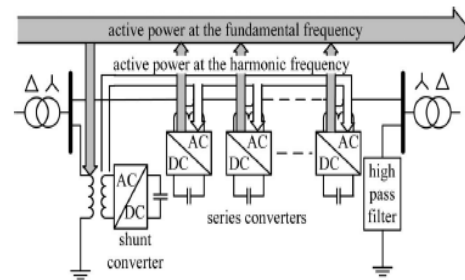
Fig. 4. Active power exchange between DPFC converters.
