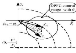
Fig. 11. Relationship between P_{se,1} and the power flow at the receiving end.
