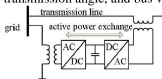
Fig. 1. Simplified representation of a UPFC.
