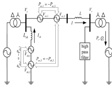
Fig. 8. DPFC simplified representation
