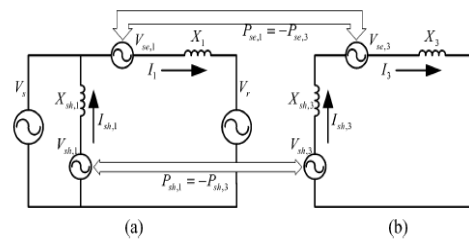
Fig. 9. DPFC equivalent circuit. (a) Fundamental Frequency. (b) Third-Harmonic Frequency.
