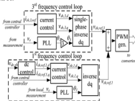
Fig. 16. Block diagram of the shunt converter control.
