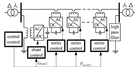
Fig. 14. DPFC control block diagram.
