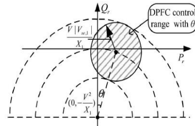
Fig. 10. DPFC active and reactive power control range with the transmission angle
