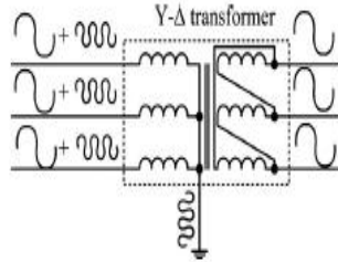
Fig.5. Utilize grounded Y-Δ transformer to provide path for the zero – sequence third harmonic.
