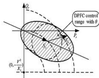
Fig. 13. DPFC power-flow control range frequencies component.
