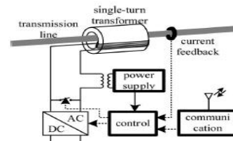
Fig. 7. D-FACTS unit configuration [7]
