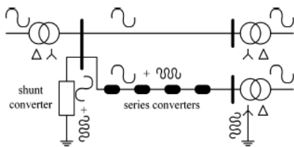
Fig.6. Route the harmonic current by using the grounding status of the Y-Δ transformer.
