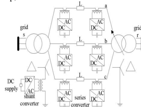
Fig.17. DPFC experimental setup circuit
