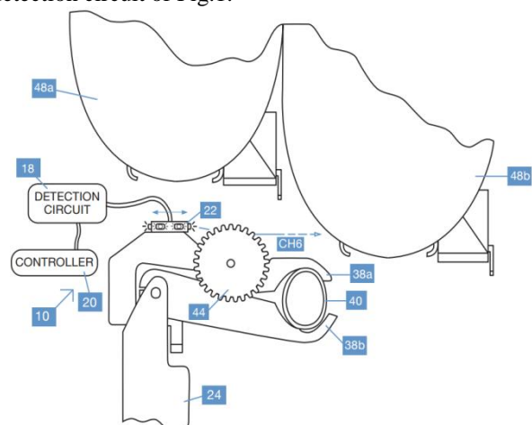
Fig.1. Gripper Design & Drawing by Dr. Rafie Hamidpour
