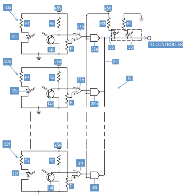
Fig.4. Circuit Design & Drawing by Dr. Rafie Hamidpour
