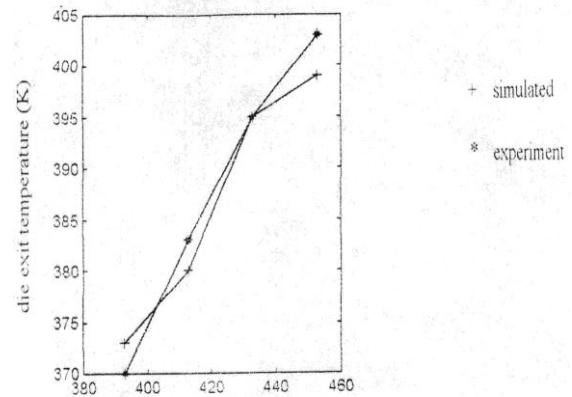
Fig.9. Simulated and experimental values for die exit temperature
