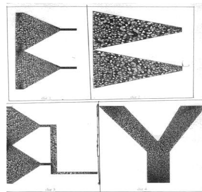
Fig.2. Meshing diagram of dies used in Flotran analysis
