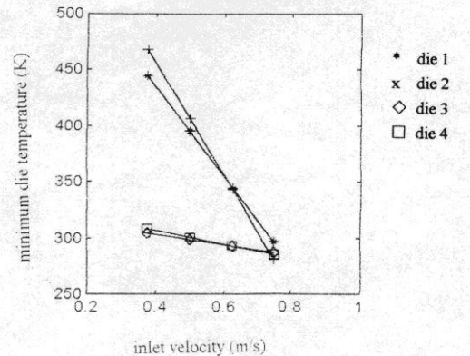
Fig.10. Relationship between inlet velocity and minimum die temperature
