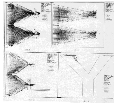
Fig.4. Velocity vector diagram for inlet velocity of 0.625 m/s
