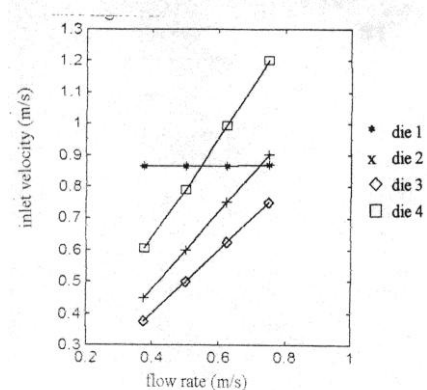
Fig.5. Relationship between the flow velocity and inlet velocity for different dies
