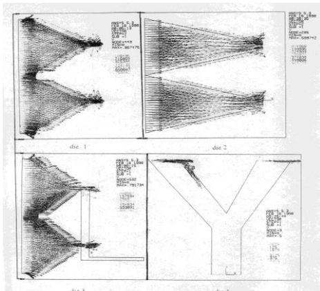
Fig.3. Velocity vector diagram at inlet velocity of 0.5m/s
