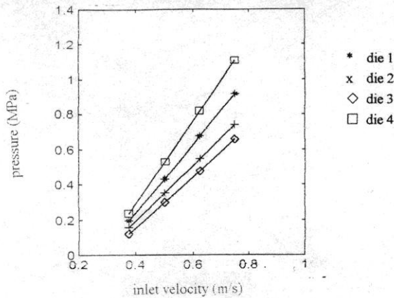
Fig.11. Relationship between inlet velocity and pressure at 0.5 m/s and 433K
