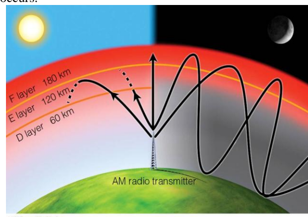
Fig. 3.1 the Ionosphere
