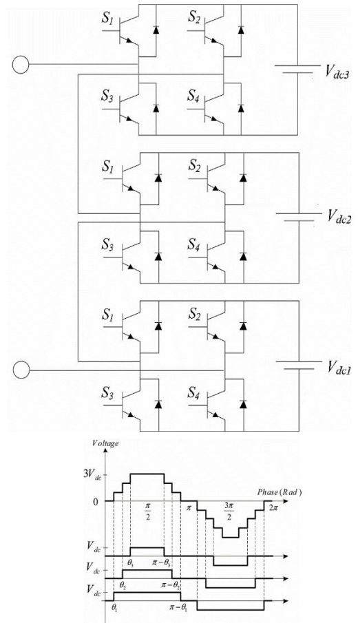
Figure 1: Structure of series H-bridge inverter: (7-levels inverter with its output waveforms)
