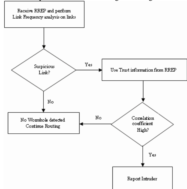
Fig.2. Flowchart for detection of Active attack
